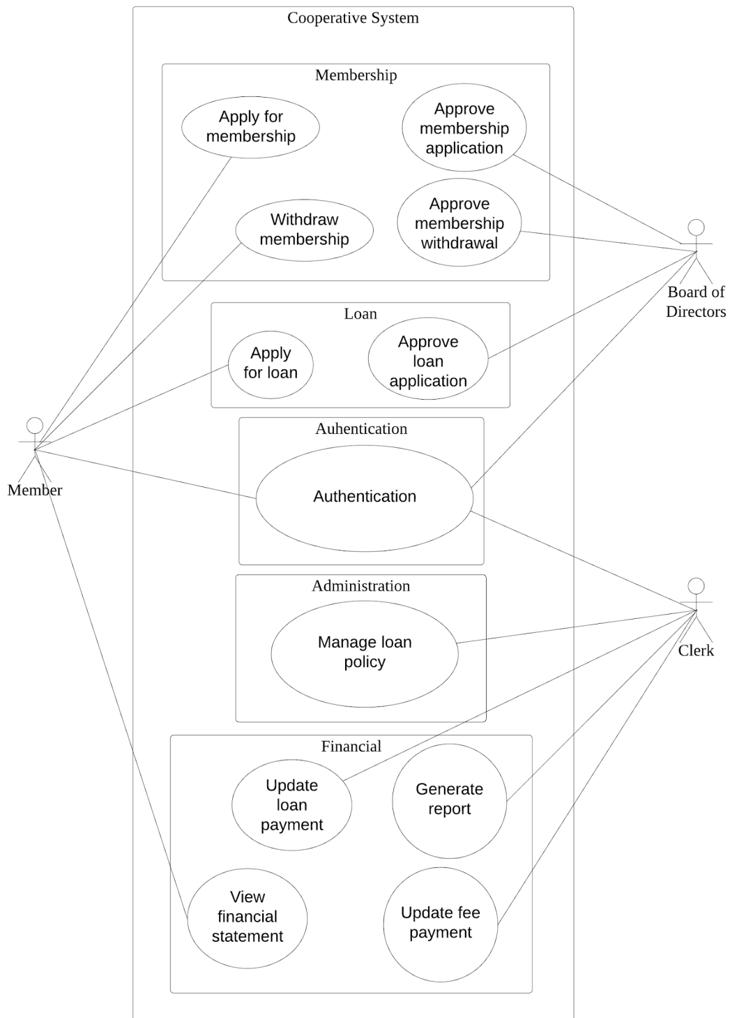
Figure 1: Use Case Diagram for KADA's Cooperative Web-Based System
